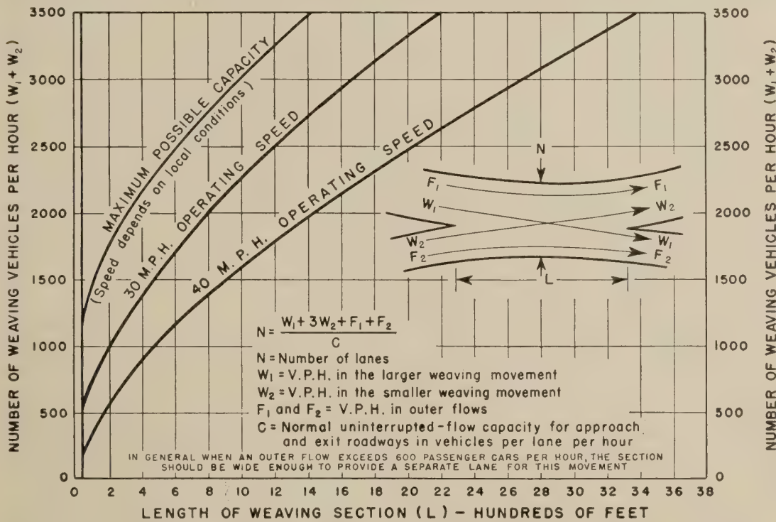
Figure 43.—Operating characteristics of weaving sections.
